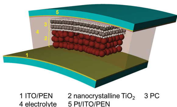
Figure 1. Schematic of 1DPC integrated flexible DSCs. The 1DPC, composing of individual layers of small TiO 2 and SiO 2 , was deposited onto nanocrystalline TiO 2 (nc-TiO 2 ) with solution process. The substrates are plastics (PEN) with ITO conducting layer coated as working electrode and Pt/ITO coated at counter electrode. The 1DPC integrated nc-TiO 2 electrode was immersed in electrolyte, which was injected into the space between two flexible substrates.
