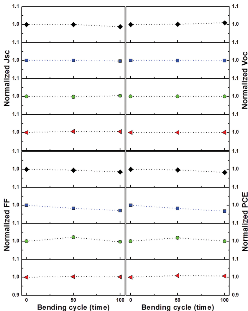
Figure 6. Photovoltaic performance of cells under repeated bending for 0, 50, and 100 times with bending radius of 14 mm. The J_{SC} , V_{OC} , FF, and PCE of cells are normalized by comparing with that before bending. Different color lines are used for the reference cell (black line), and for cells in which the electrodes are coated with blue, green, and red light reflecting 1DPCs (blue, green, and red lines, respectively).
